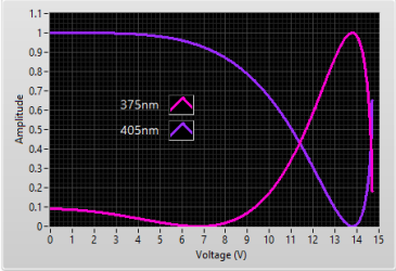
G8192 Intensity-Voltage Response
