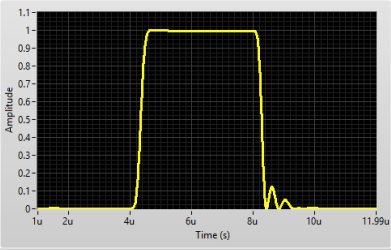
G8192 Pulse Response
